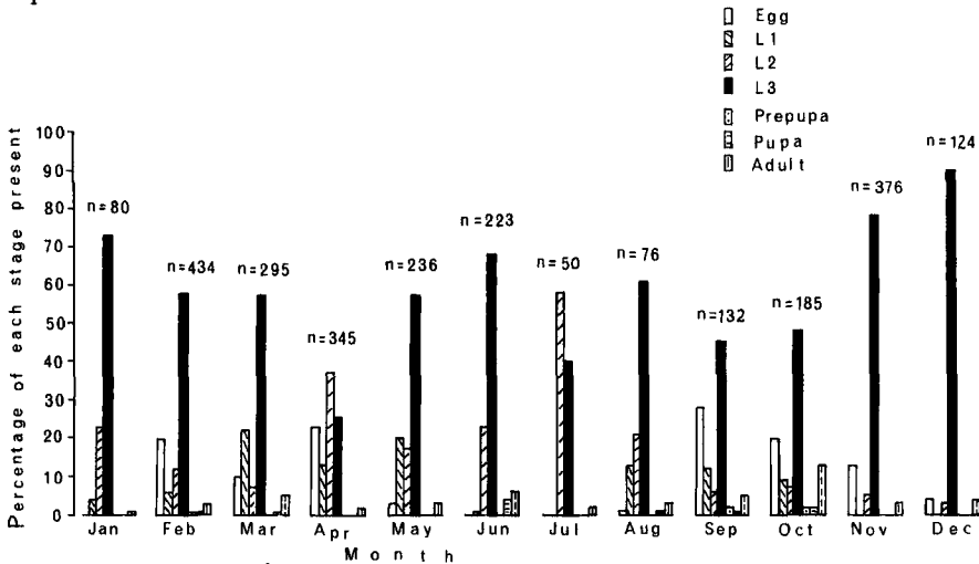
FIG. 2.—Histogram showing percentage of different stages of O. rhinoceros found in tops of dead standing palms at Malapau during the year. (n = total of all stages.)
